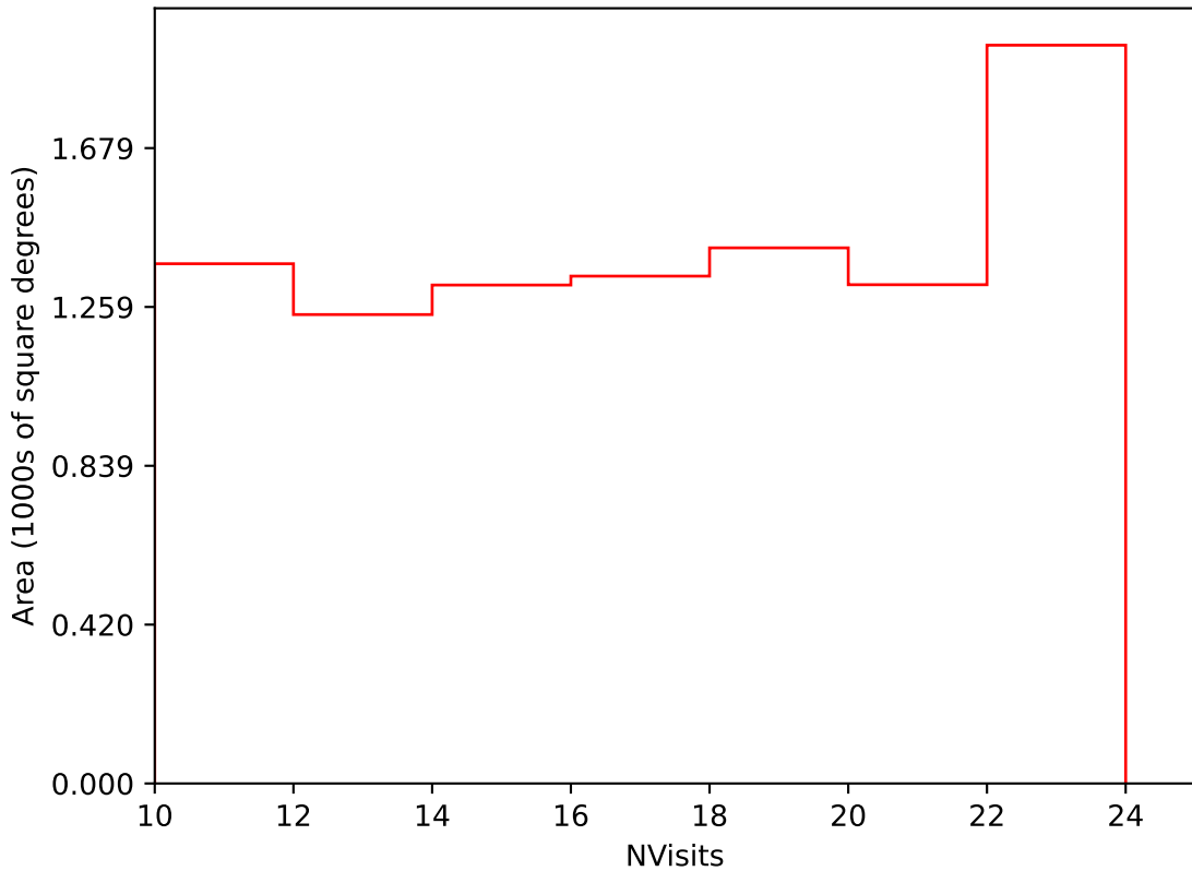
ddf_loaded_half_fl1_v3.4_10yrs Yr 3-4 i band: NVisits
