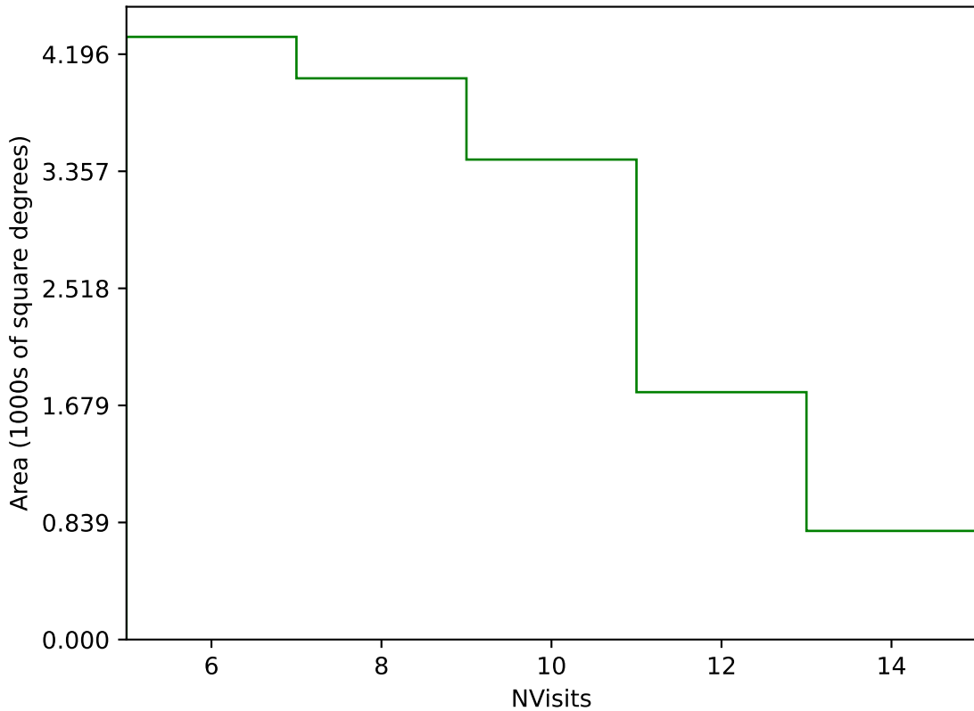
ddf_loaded_half_fl1_v3.4_10yrs Yr 3-4 g band: NVisits
