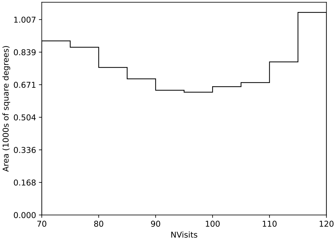
ddf_loaded_half_fl1_v3.4_10yrs Yr 3-4 all bands: NVisits
