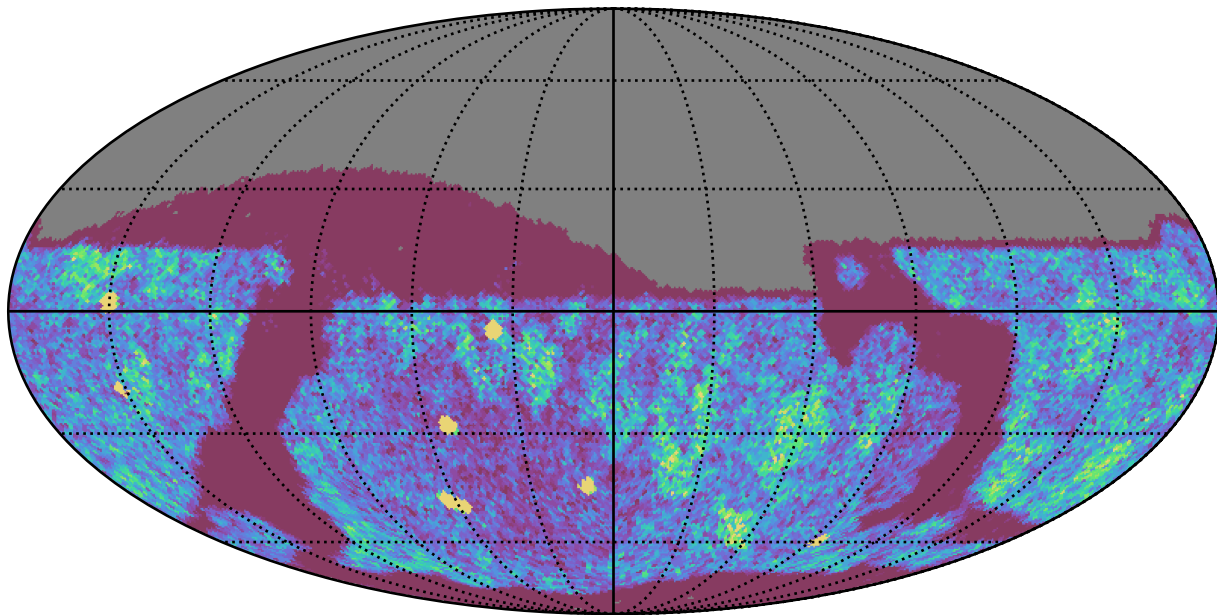
ddf_loaded_half_fl1_v3.4_10yrs Yr 1 z band: NVisits
