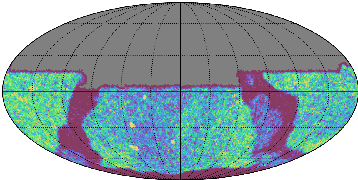
ddf_loaded_half_fl1_v3.4_10yrs Yr 1 y band: NVisits
