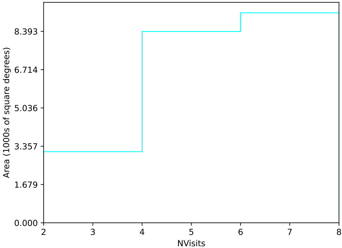
ddf_loaded_half_fl1_v3.4_10yrs Yr 1 u band: NVisits
