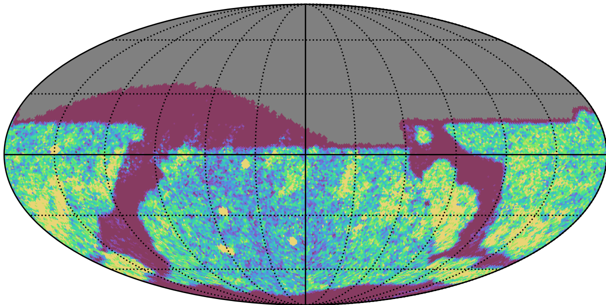
ddf_loaded_half_fl1_v3.4_10yrs Yr 1 r band: NVisits
