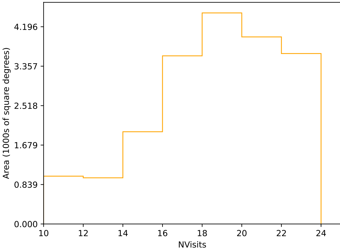
ddf_loaded_half_fl1_v3.4_10yrs Yr 1 r band: NVisits
