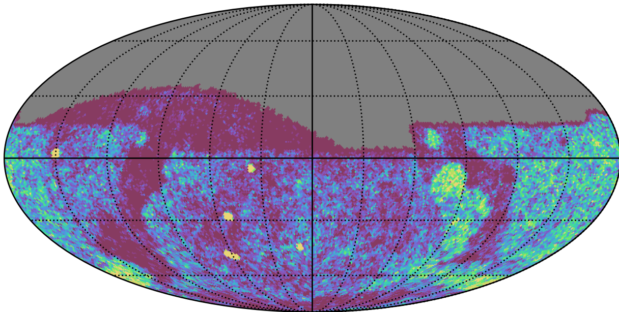
ddf_loaded_half_fl1_v3.4_10yrs Yr 1 g band: NVisits
