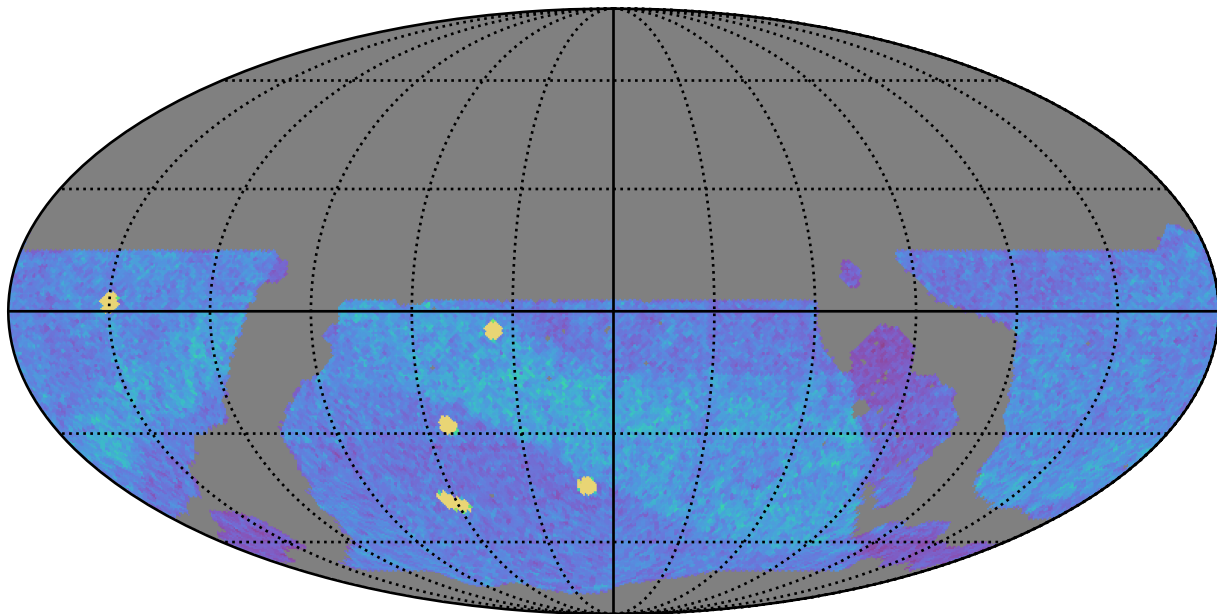
ddf_loaded_half_fl1_v3.4_10yrs WFD z band: NVisits
