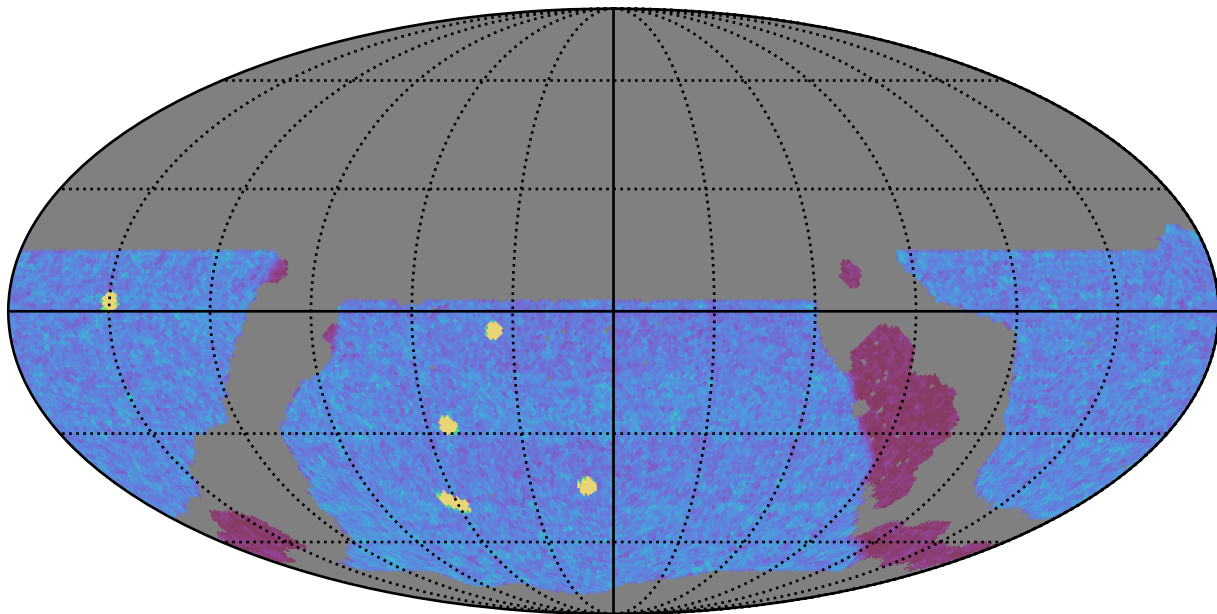
ddf_loaded_half_fl1_v3.4_10yrs WFD y band: NVisits
