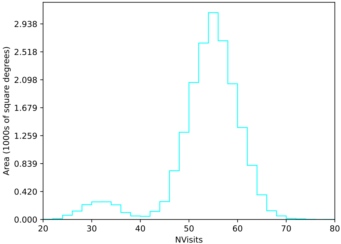
ddf_loaded_half_fl1_v3.4_10yrs WFD u band: NVisits
