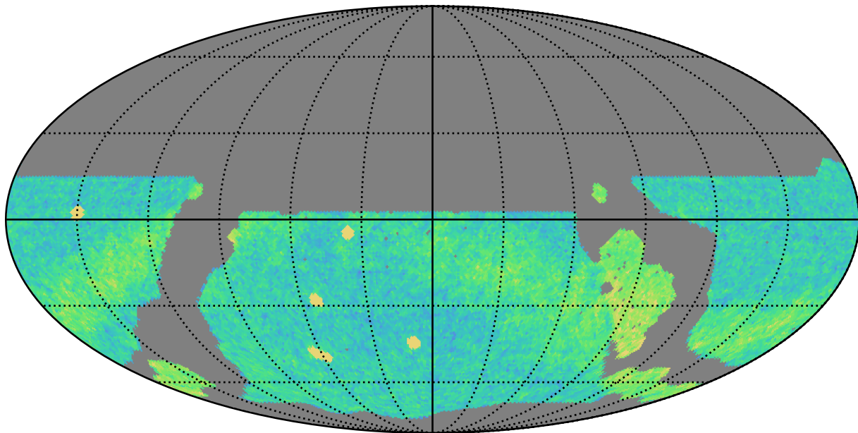
ddf_loaded_half_fl1_v3.4_10yrs WFD r band: NVisits
