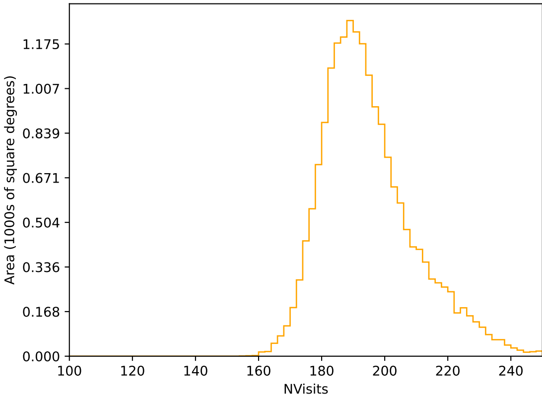
ddf_loaded_half_fl1_v3.4_10yrs WFD r band: NVisits
