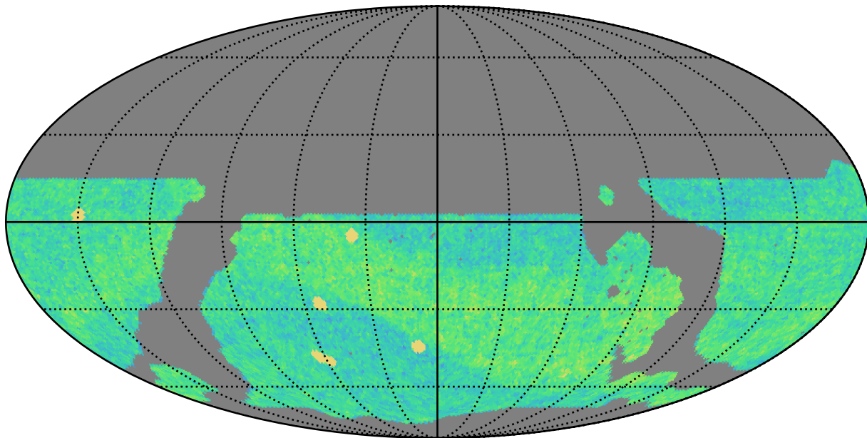
ddf_loaded_half_fl1_v3.4_10yrs WFD i band: NVisits
