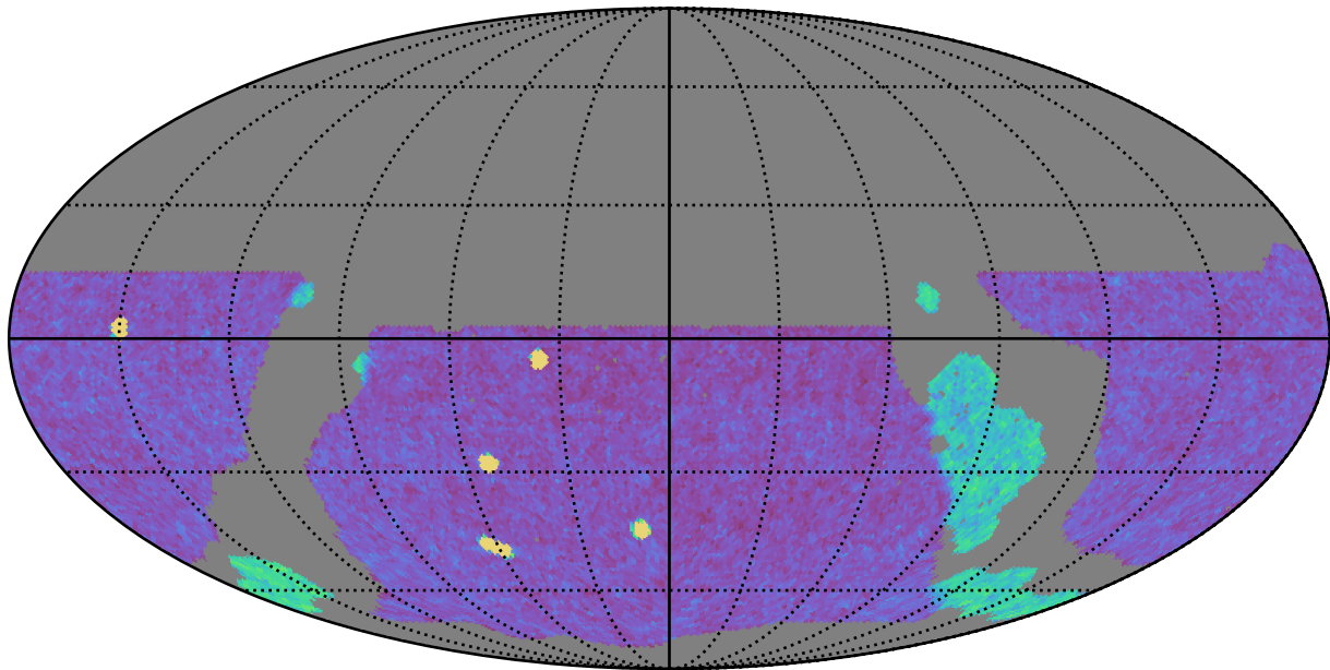
ddf_loaded_half_fl1_v3.4_10yrs WFD g band: NVisits
