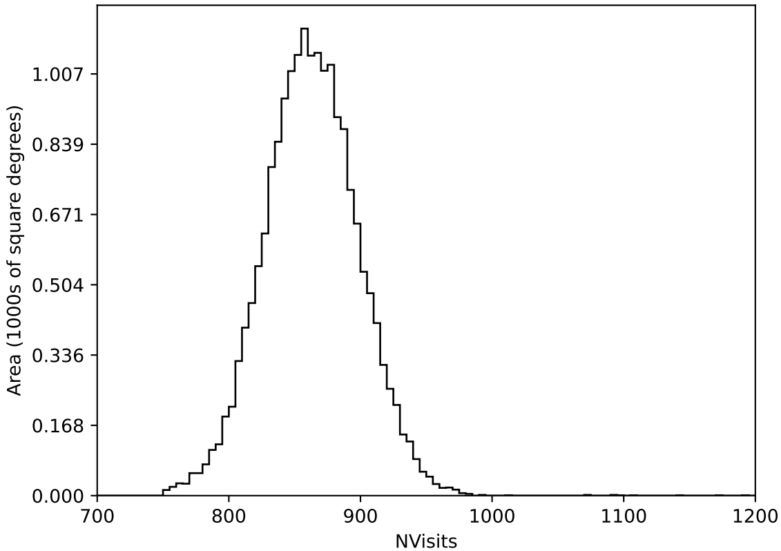
ddf_loaded_half_fl1_v3.4_10yrs WFD all bands: NVisits
