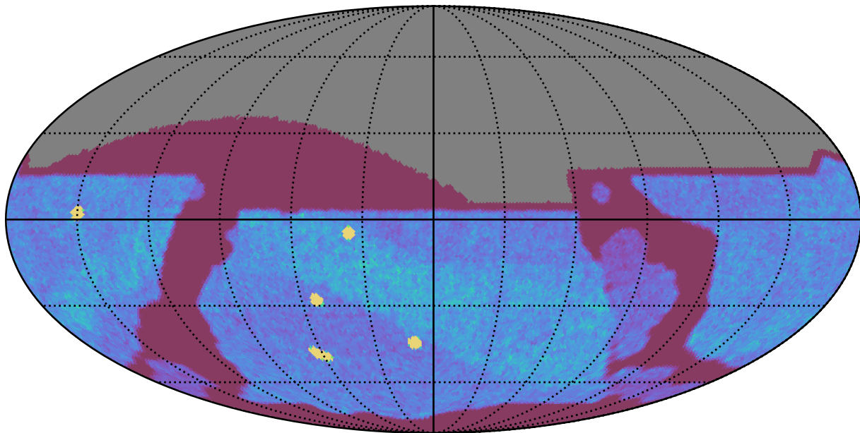
ddf_loaded_half_fl1_v3.4_10yrs All sky z band: NVisits
