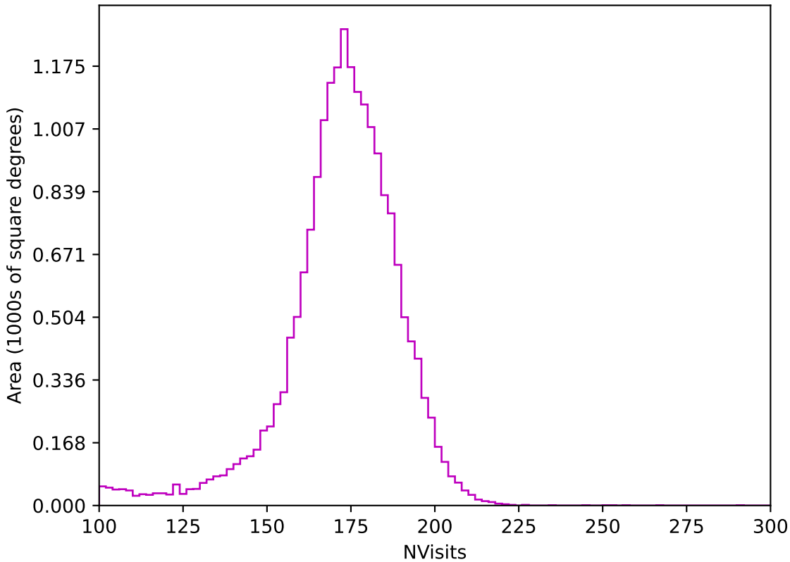
ddf_loaded_half_fl1_v3.4_10yrs All sky z band: NVisits
