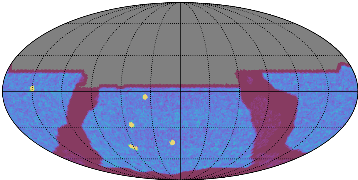
ddf_loaded_half_fl1_v3.4_10yrs All sky y band: NVisits
