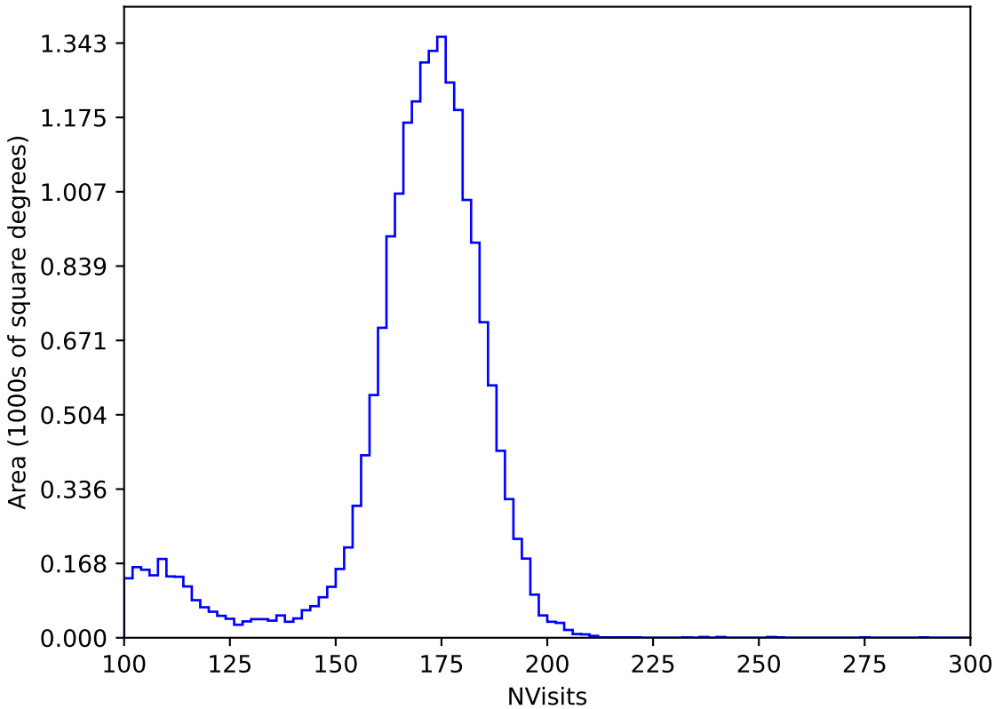
ddf_loaded_half_fl1_v3.4_10yrs All sky y band: NVisits
