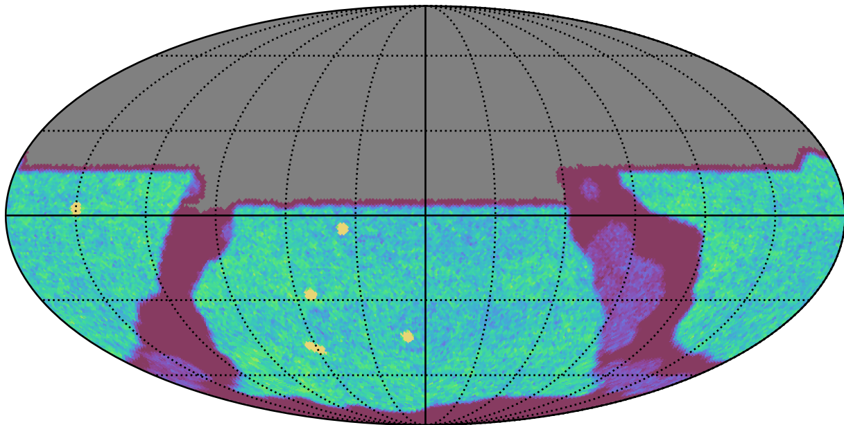
ddf_loaded_half_fl1_v3.4_10yrs All sky u band: NVisits
