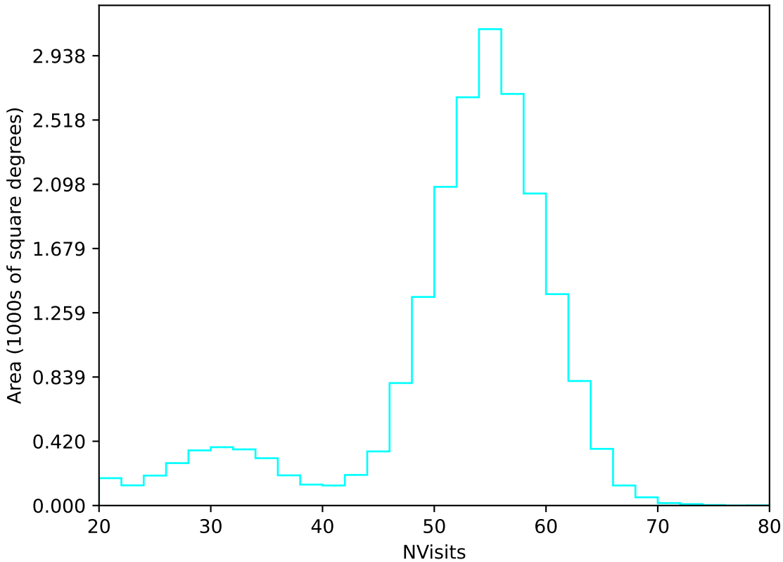
ddf_loaded_half_fl1_v3.4_10yrs All sky u band: NVisits
