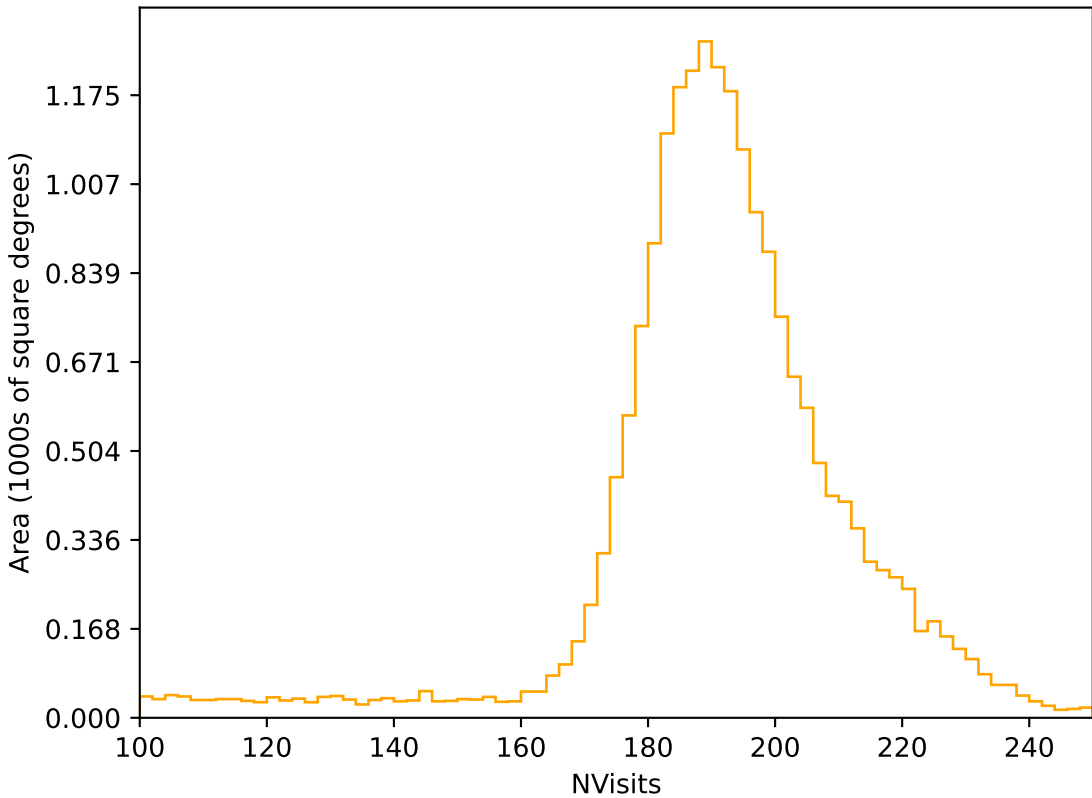
ddf_loaded_half_fl1_v3.4_10yrs All sky r band: NVisits
