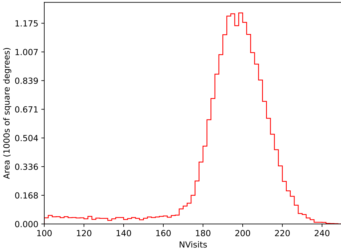
ddf_loaded_half_fl1_v3.4_10yrs All sky i band: NVisits
