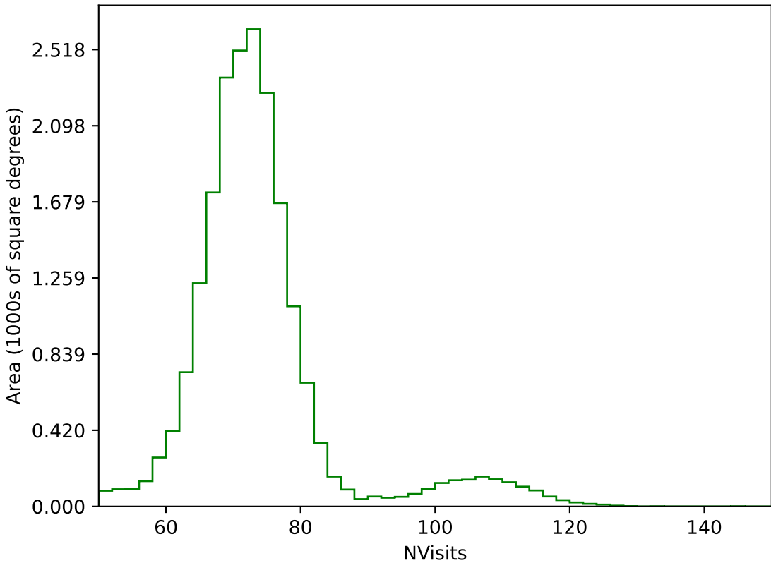
ddf_loaded_half_fl1_v3.4_10yrs All sky g band: NVisits
