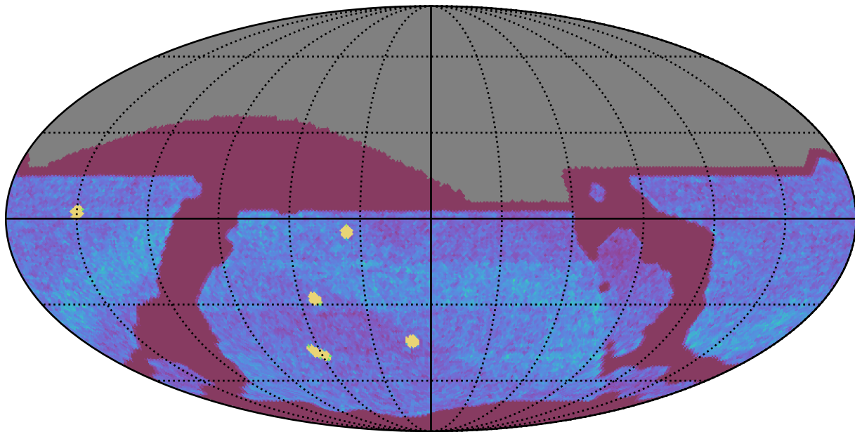
ddf_loaded_half_f11_v3.4_10yrs All sky all bands: NVisits
