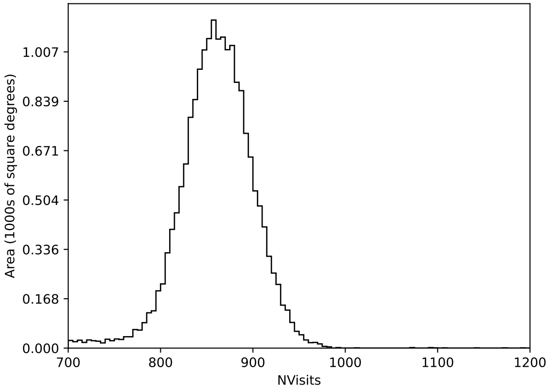
ddf_loaded_half_fl1_v3.4_10yrs All sky all bands: NVisits
