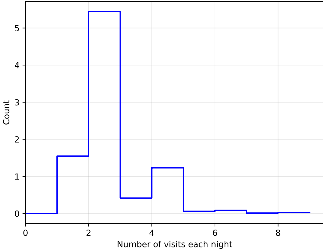
ddf_loaded_half_fl1_v3.4_10yrs WFD: NVisitsPerNight
