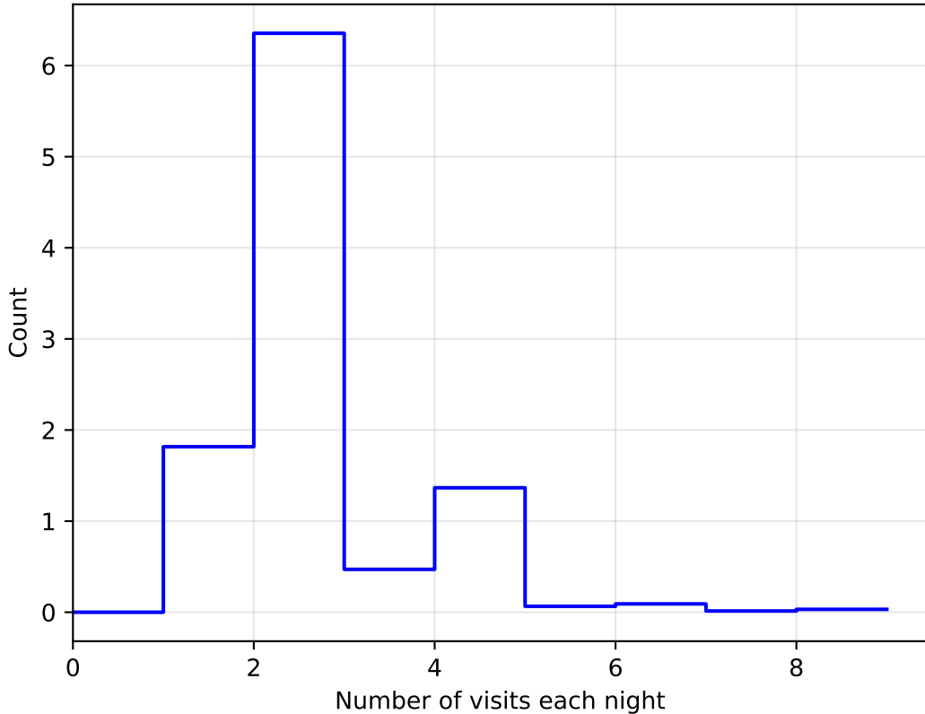
ddf_loaded_half_fl1_v3.4_10yrs All sky: NVisitsPerNight
