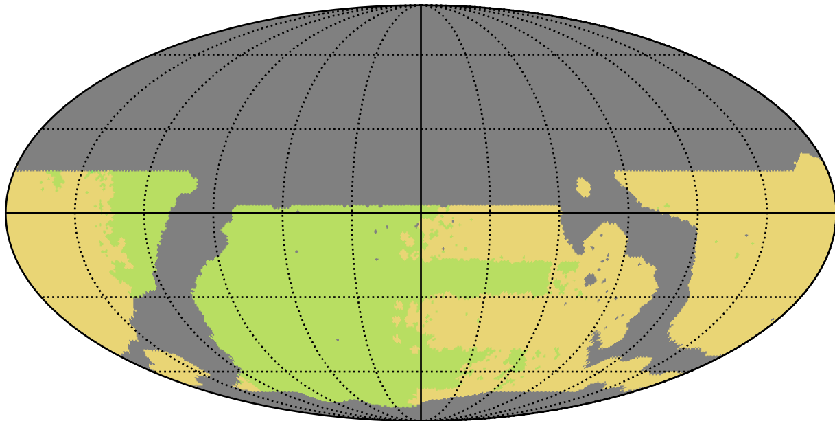
ddf_loaded_half_fl1_v3.4_10yrs WFD all bands: NSeasons
