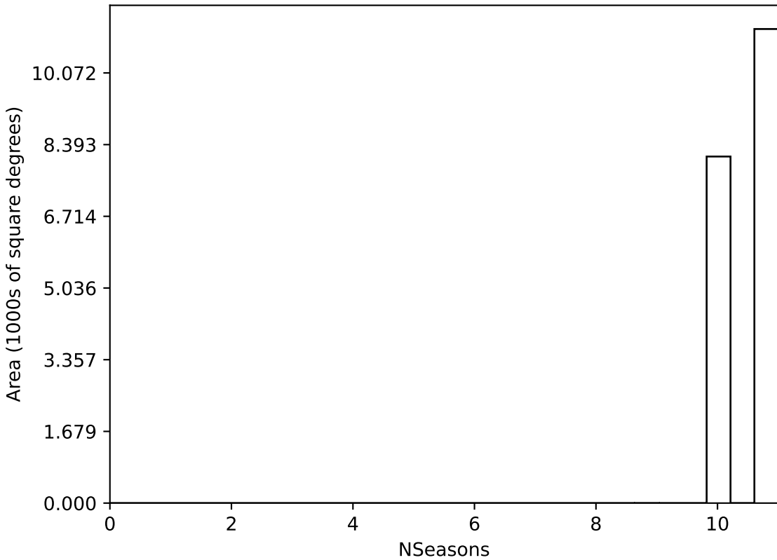
ddf_loaded_half_fl1_v3.4_10yrs WFD all bands: NSeasons
