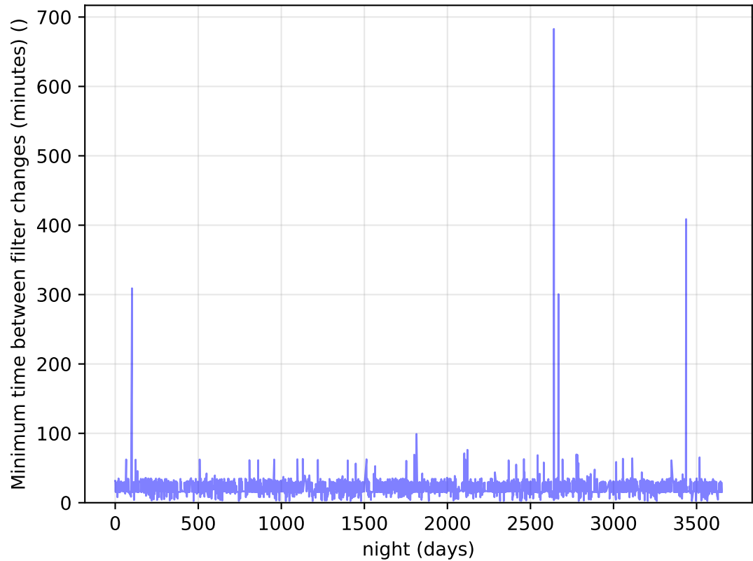
ddf_loaded_half_fl1_v3.4_10yrs Per Night: Minimum time between filter changes (minutes)
