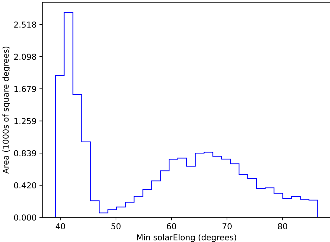
ddf_loaded_half_fl1_v3.4_10yrs WFD r band: Min solarElong
