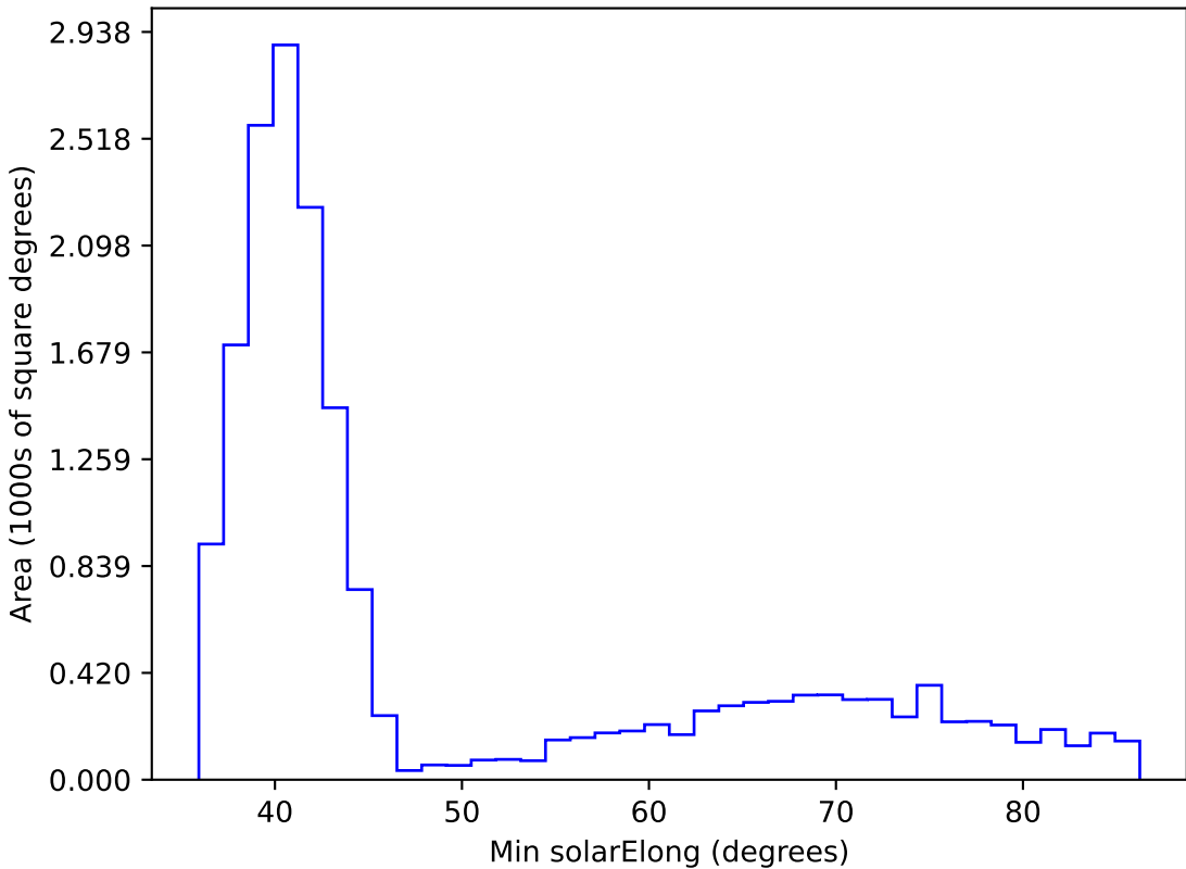
ddf_loaded_half_fl1_v3.4_10yrs WFD i band: Min solarElong
