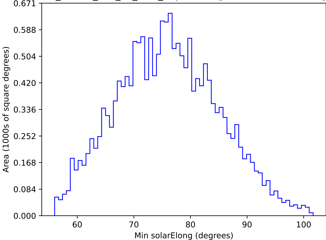
ddf_loaded_half_fl1_v3.4_10yrs WFD g band: Min solarElong
