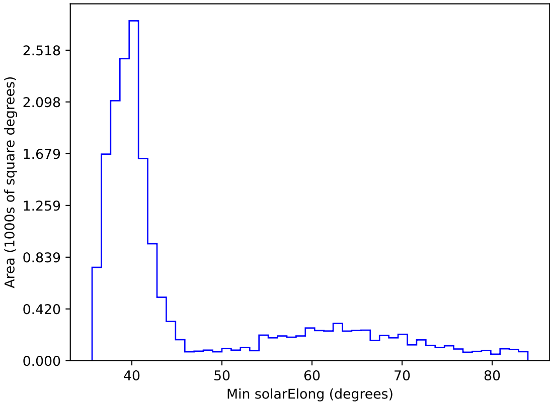
ddf_loaded_half_fl1_v3.4_10yrs WFD all bands: Min solarElong
