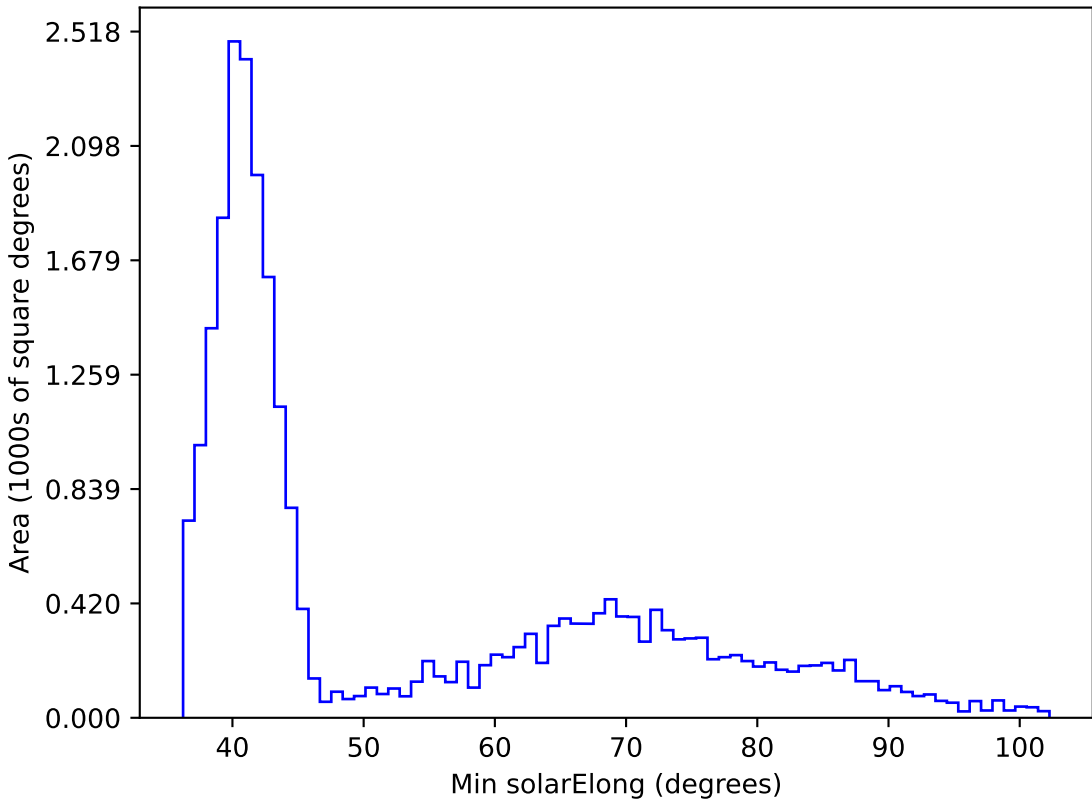
ddf_loaded_half_fl1_v3.4_10yrs All sky z band: Min solarElong
