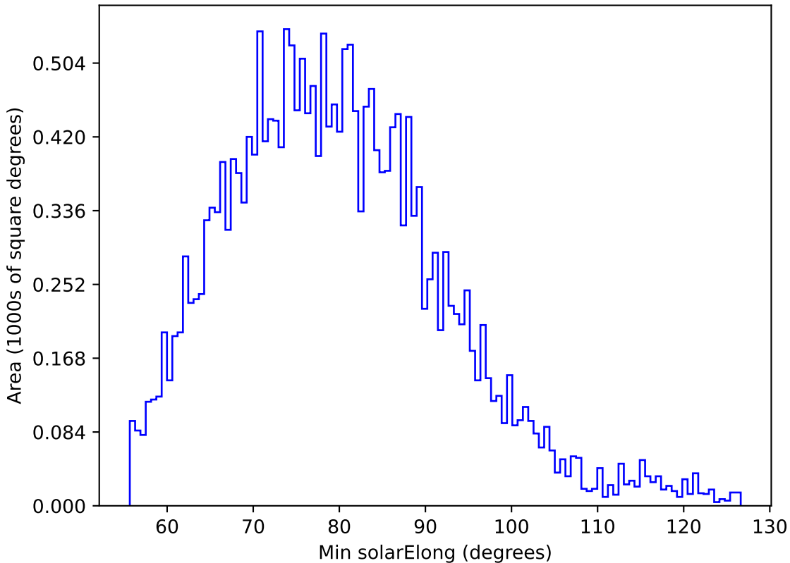
ddf_loaded_half_fl1_v3.4_10yrs All sky u band: Min solarElong
