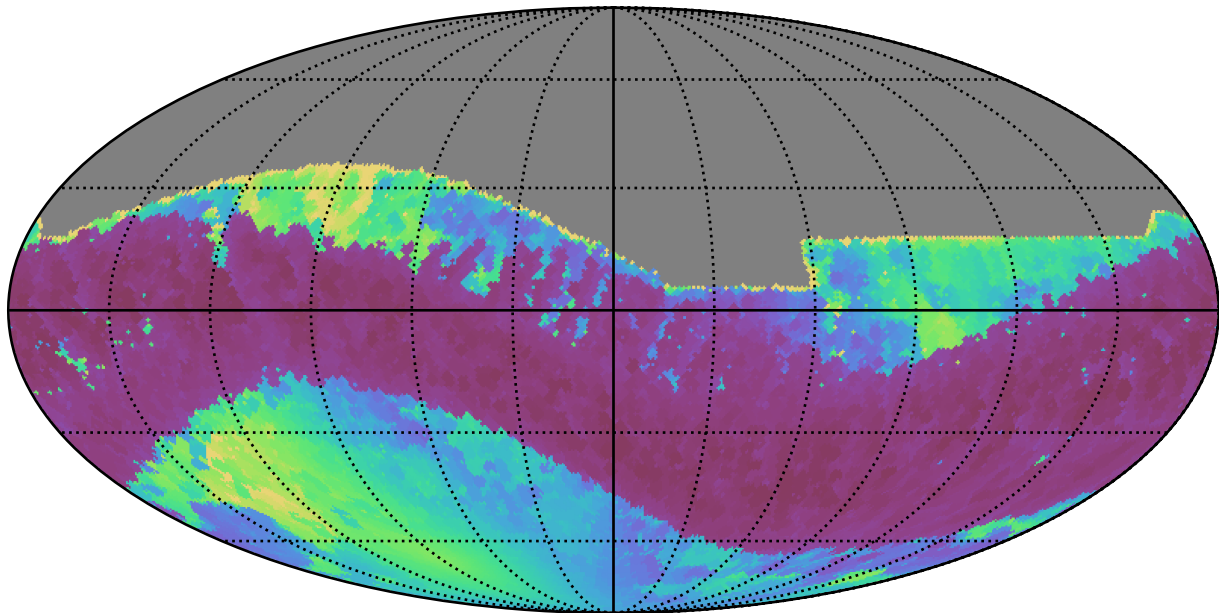
ddf_loaded_half_fl1_v3.4_10yrs All sky i band: Min solarElong
