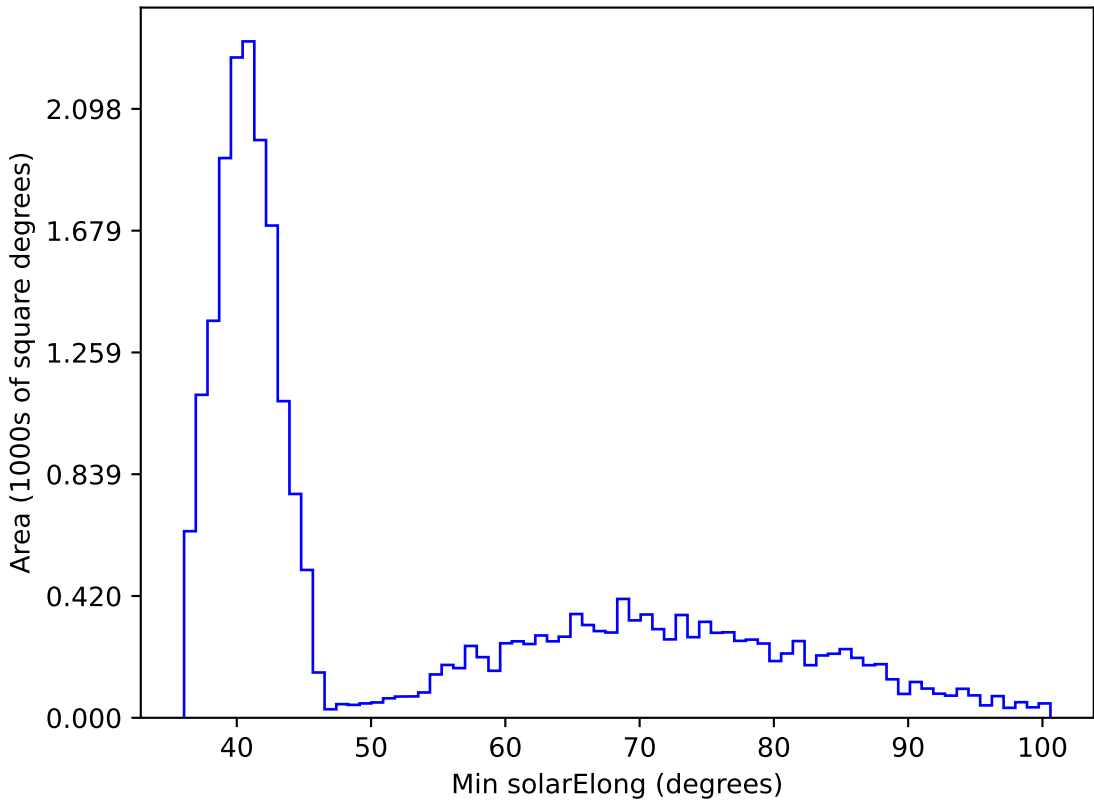
ddf_loaded_half_fl1_v3.4_10yrs All sky i band: Min solarElong
