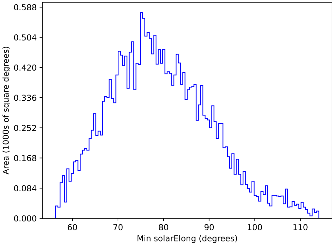
ddf_loaded_half_fl1_v3.4_10yrs All sky g band: Min solarElong
