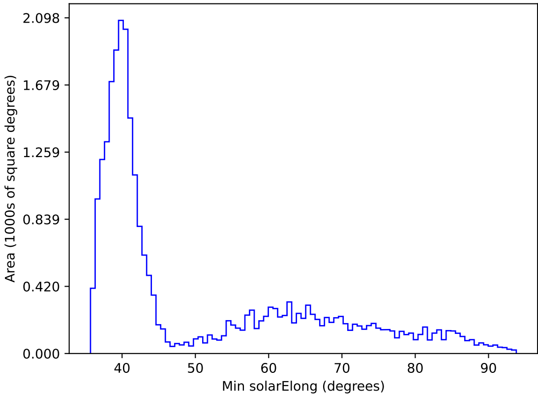
ddf_loaded_half_fl1_v3.4_10yrs All sky all bands: Min solarElong
