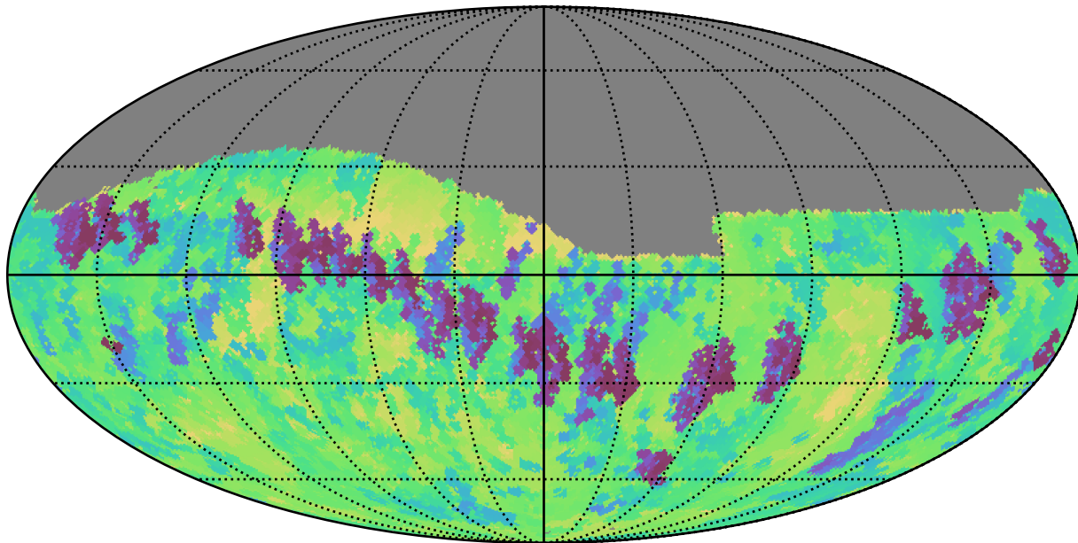
ddf_loaded_half_fl1_v3.4_10yrs Yr 1 z band: Min skyBrightness
