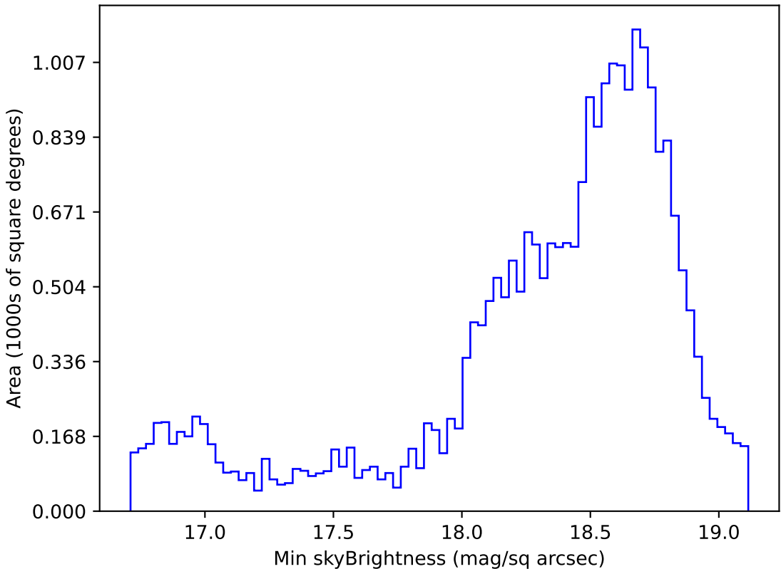
ddf_loaded_half_fl1_v3.4_10yrs Yr 1 z band: Min skyBrightness
