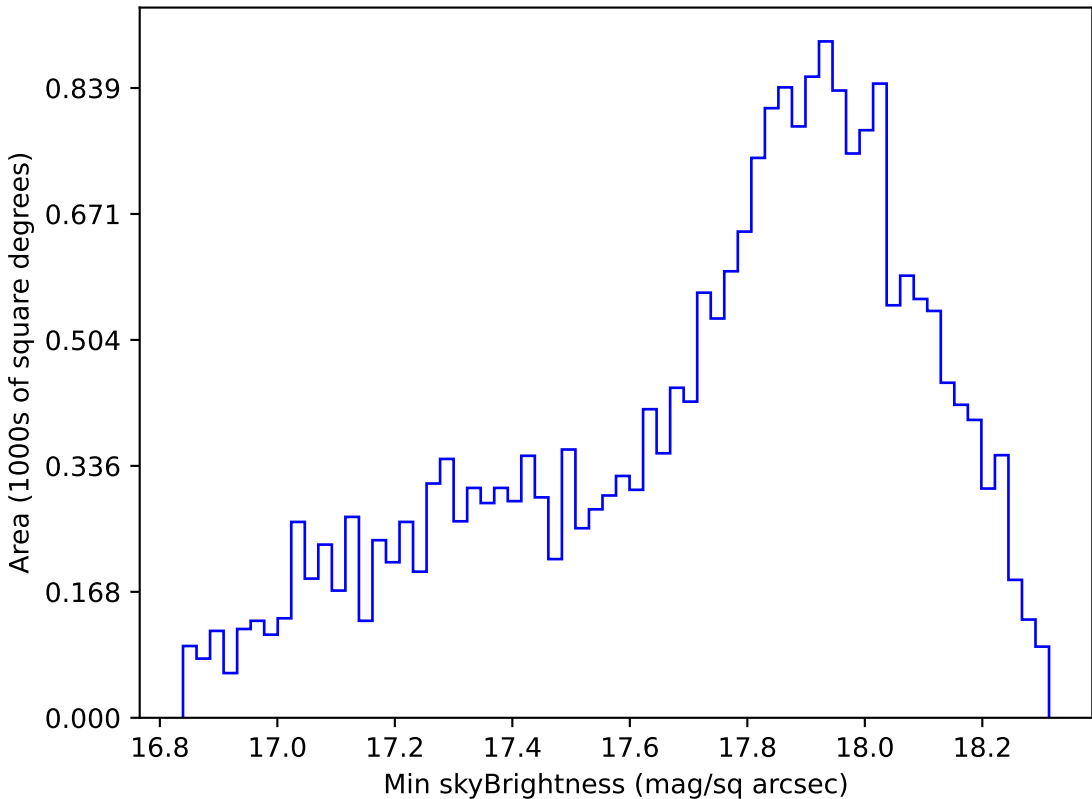
ddf_loaded_half_fl1_v3.4_10yrs Yr 1 y band: Min skyBrightness
