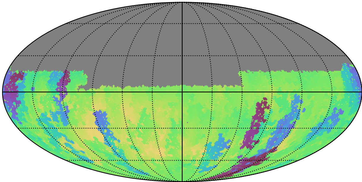
ddf_loaded_half_fl1_v3.4_10yrs Yr 1 u band: Min skyBrightness
