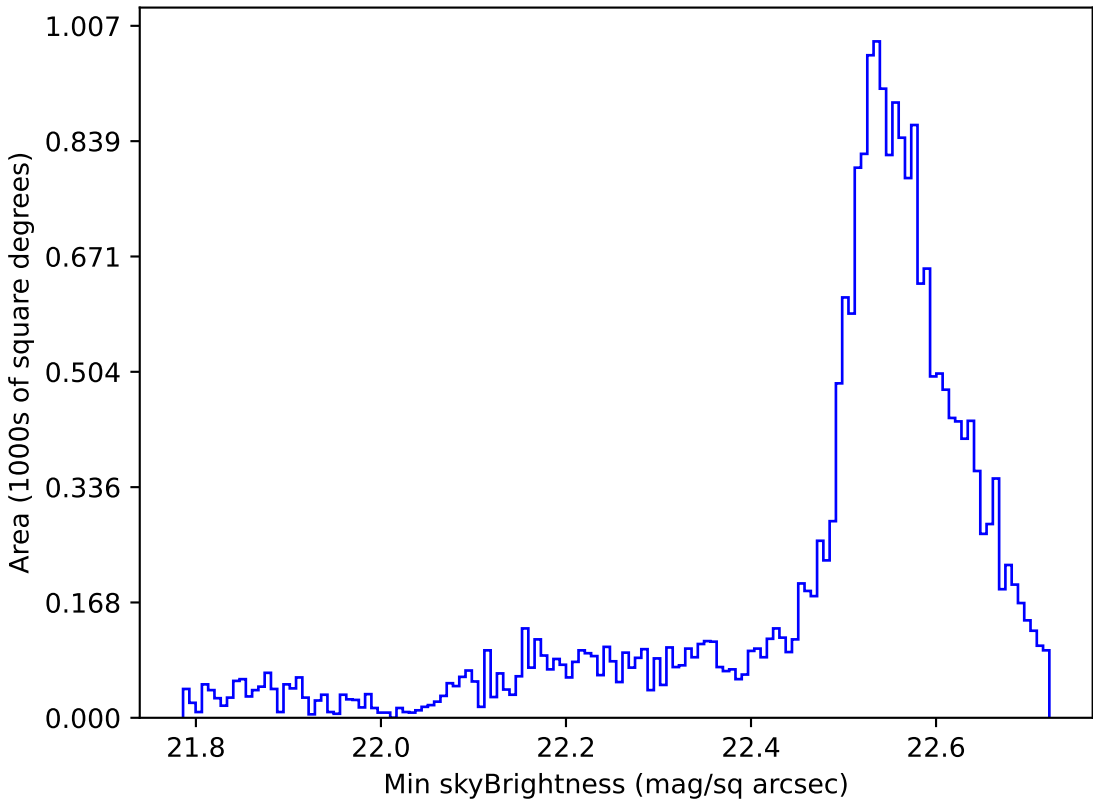
ddf_loaded_half_fl1_v3.4_10yrs Yr 1 u band: Min skyBrightness
