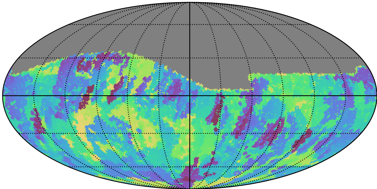
ddf_loaded_half_fl1_v3.4_10yrs Yr 1 r band: Min skyBrightness
