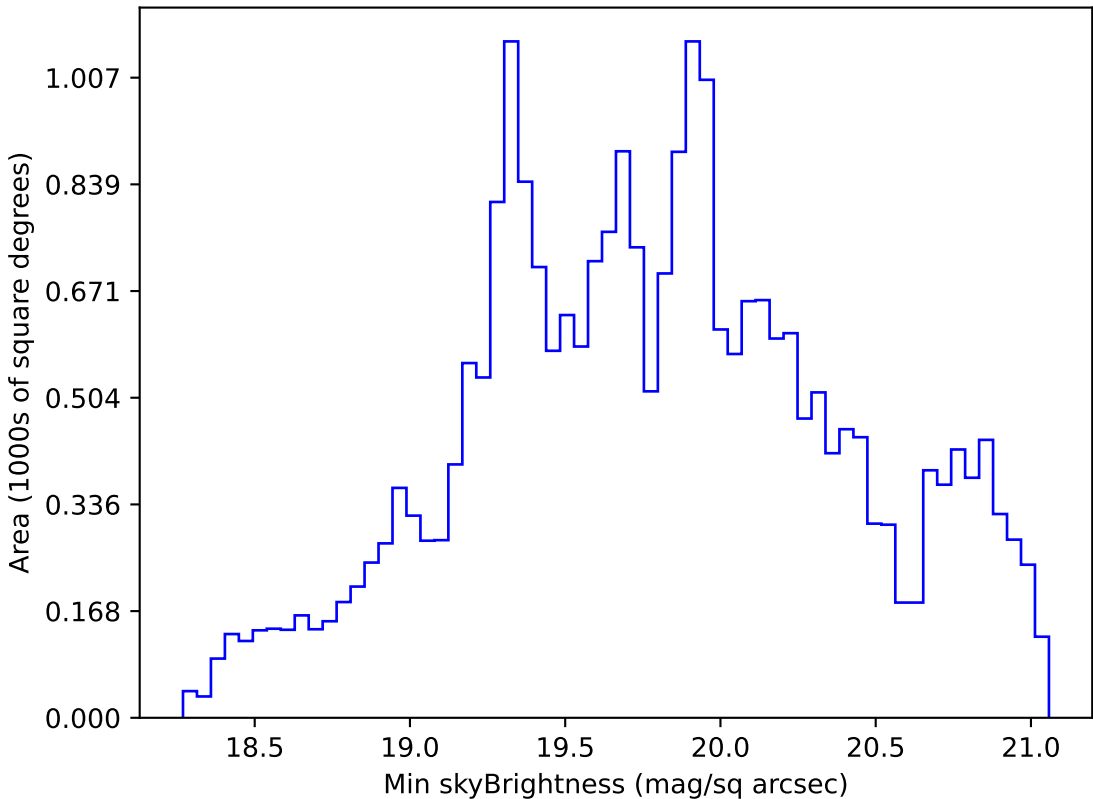
ddf_loaded_half_fl1_v3.4_10yrs Yr 1 r band: Min skyBrightness
